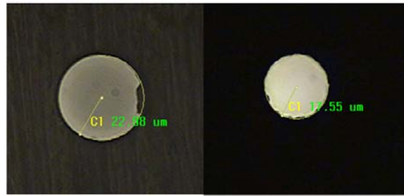
(a) 45μm hole entrance (b) 35μm hole exit
